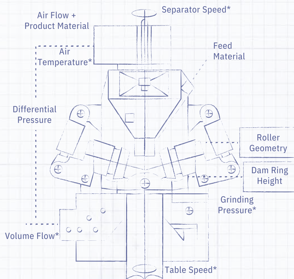
Fig.4 Cement Vertical Roller Mill
