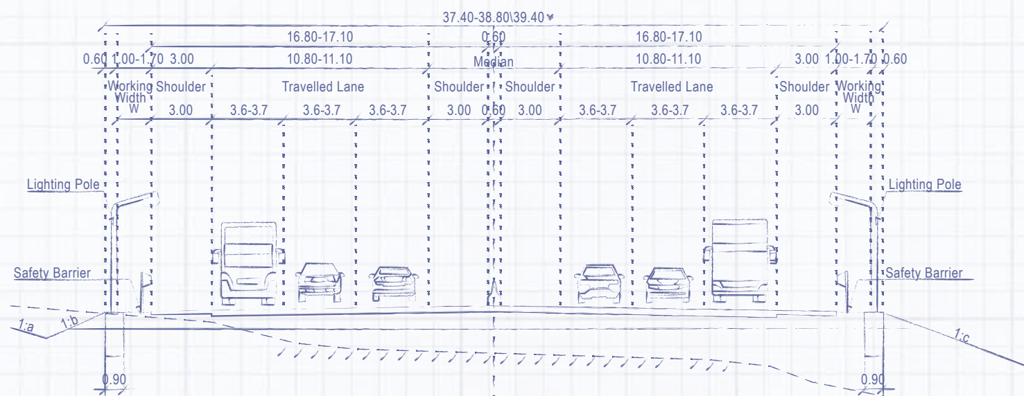
Fig.2 6-lane Expressway Cross Section
